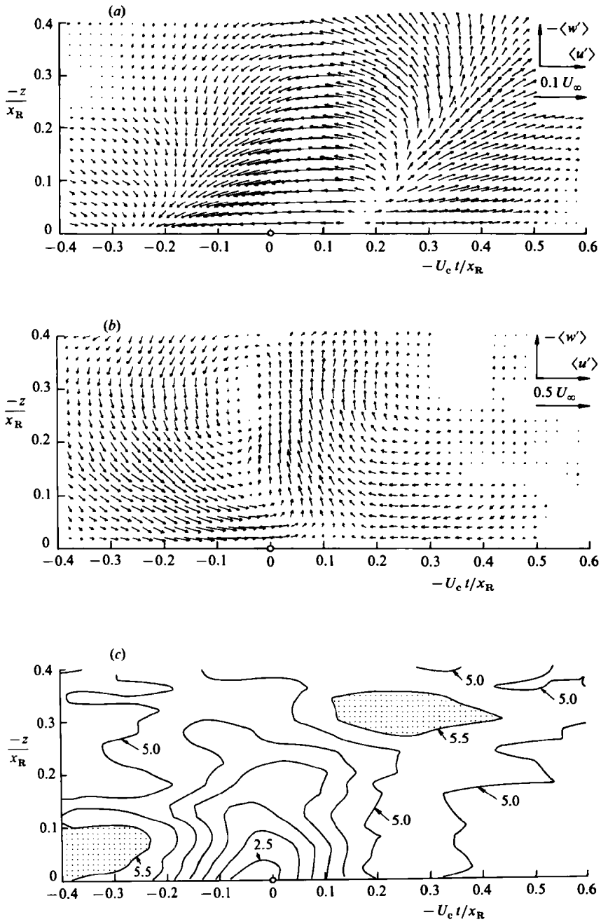
FIGURE 7. Space-time ( z, t ) distributions of fluctuating velocity vector ( \langle u' \rangle, \langle w' \rangle ) at height (a) y/x_R = 0.32 and (b) 0.16 and (c) contour lines of high-frequency energy \langle u_T'^2 \rangle in a normalized form 10^4 \langle u_T'^2 \rangle / U_\infty^2 (contour interval 0.5 ), shaded areas being areas where the normalized energy is higher than 5.5 . Time t is synchronized with peaks of p'_R .
