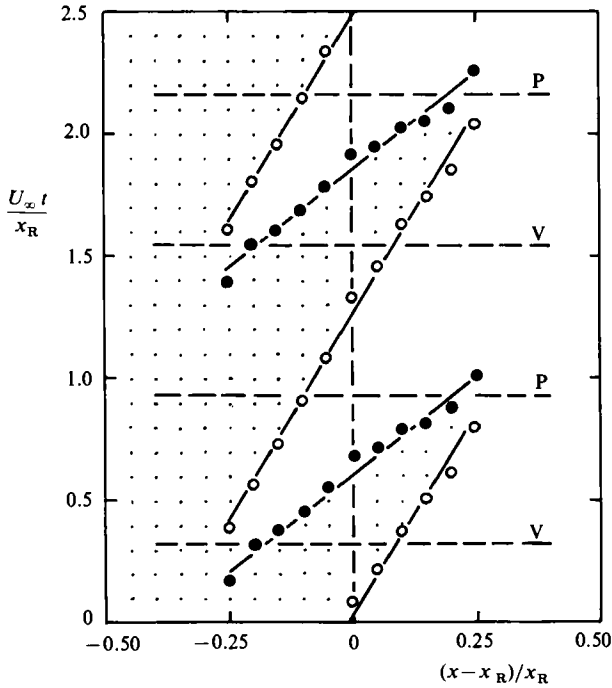
FIGURE 13. Motion of zeros A and B of the surface velocity in the space-time (x-x_R, t) domain: broken horizontal lines denoted by P and V indicate the time at which the phase-averaged pressure fluctuation \langle p'_R \rangle attains a peak and a valley, respectively; \circ , A ; \bullet , B ; shaded area is reverse-flow region; origin of time t is arbitrary.
