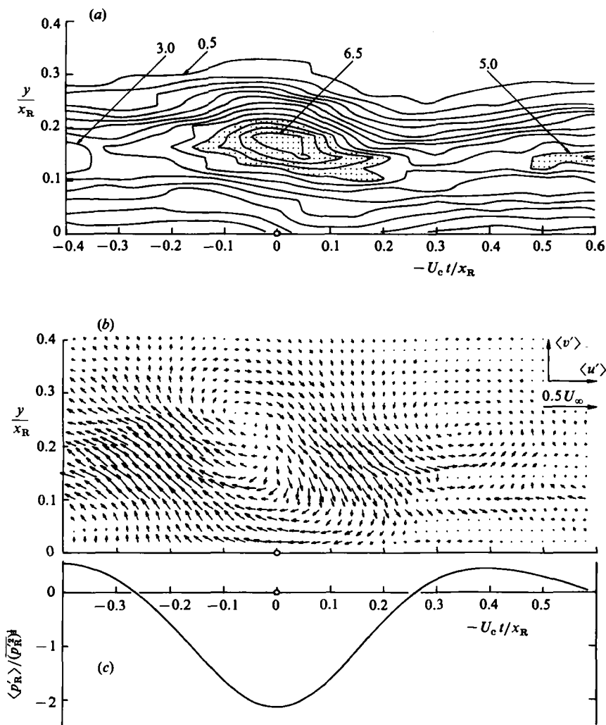
FIGURE 4. Space-time (y, t) distributions of (a) contour lines of high-frequency turbulent energy \langle u_T'^2 \rangle in a normalized form 10^4 \langle u_T'^2 \rangle / U_\infty^2 (contour interval 0.5), shaded areas being areas where the normalized energy is higher than 0.5, (b) fluctuating velocity vector (\langle u' \rangle, \langle v' \rangle) and (c) surface-pressure fluctuation at the reattachment point \langle p_R' \rangle . Time t is synchronized with valleys of p_R' . Measurements were made in the mid-span plane. The threshold level for the valleys was -1.8 \sqrt{\langle p_R'^2 \rangle} and its detection frequency was 43 Hz which is approximately \frac{1}{3} times the vortex-shedding frequency.
