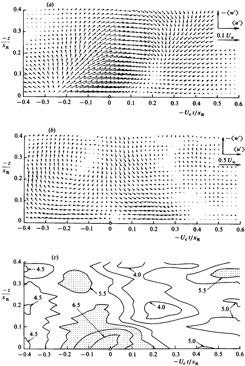
FIGURE 6. Space-time ( z, t ) distributions of fluctuating velocity vector ( \langle u' \rangle, \langle w' \rangle ) at height (a) y/x_R = 0.32 and (b) 0.16 and (c) contour lines of high-frequency energy \langle u_T'^2 \rangle in a normalized form 10^4 \langle u_T'^2 \rangle / U_\infty^2 (contour interval 0.5 ), shaded areas being areas where the normalized energy is higher than 5.5 . Time t is synchronized with valleys of p'_R .
