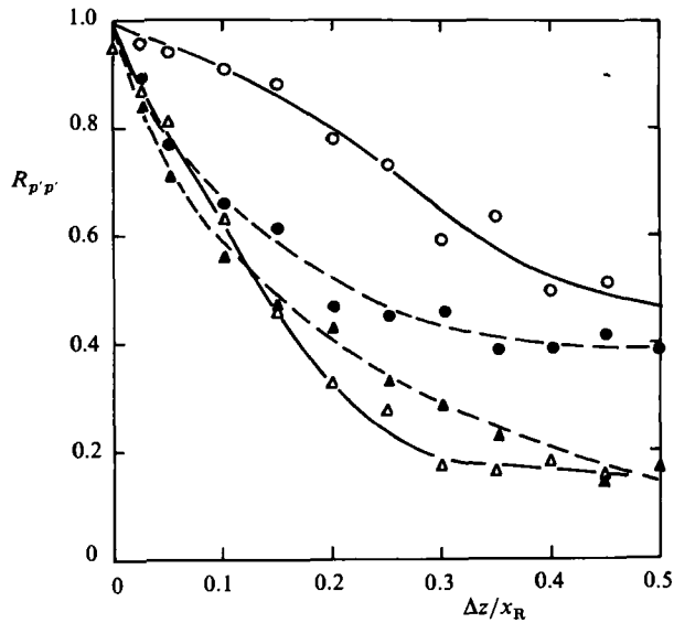
FIGURE 15. Spanwise correlation coefficients of surface-pressure fluctuations along lines x/x_R = 0.2 (open symbols \circ , \triangle ) and 1.0 (solid symbols \bullet , \blacktriangle ): one pressure transducer was fixed at the mid span and the other was traversed in the spanwise direction; \circ , \bullet , low-pass filtered component; \triangle , \blacktriangle , high-pass filtered component; the cut-off frequency was 50 Hz ( \approx 0.25U_\infty/x_R ).
