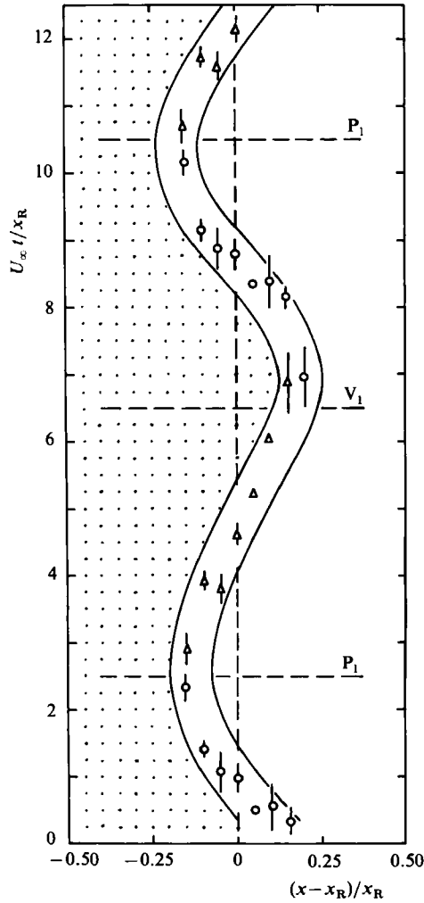
FIGURE 19. Motion of zeros A_1 and B_1 of low-pass filtered surface velocity in the space-time (x - x_R, t) domain: \Delta , A_1 ; \circ , B_1 ; flags added to symbols and solid lines represent the range of experimental uncertainty; horizontal broken lines denoted by P_1 and V_1 indicate the time at which the phase-averaged pressure \langle p'_{R1} \rangle attains peaks and valleys, respectively; the origin of time t is arbitrary; the shaded area represents a reverse-flow region.
