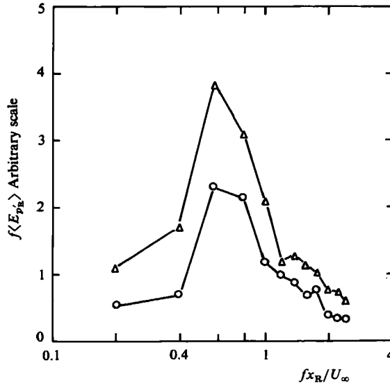
FIGURE 20. Pressure spectra for enlarged and shrunk states of separation bubble due to low-frequency unsteadiness: pressure p_1 was detected at the reattachment point; \Delta , shrunk state; \circ , enlarged state. The enlarged and shrunk states were defined by valleys V_1 and peaks P_1 of p_R . The threshold levels for the peaks and the valleys are 1.8(\overline{p_{R1}^2})^{\frac{1}{2}} and -1.8(\overline{p_{R1}^2})^{\frac{1}{2}} , the detection frequencies being 14 Hz and 11 Hz, respectively.
