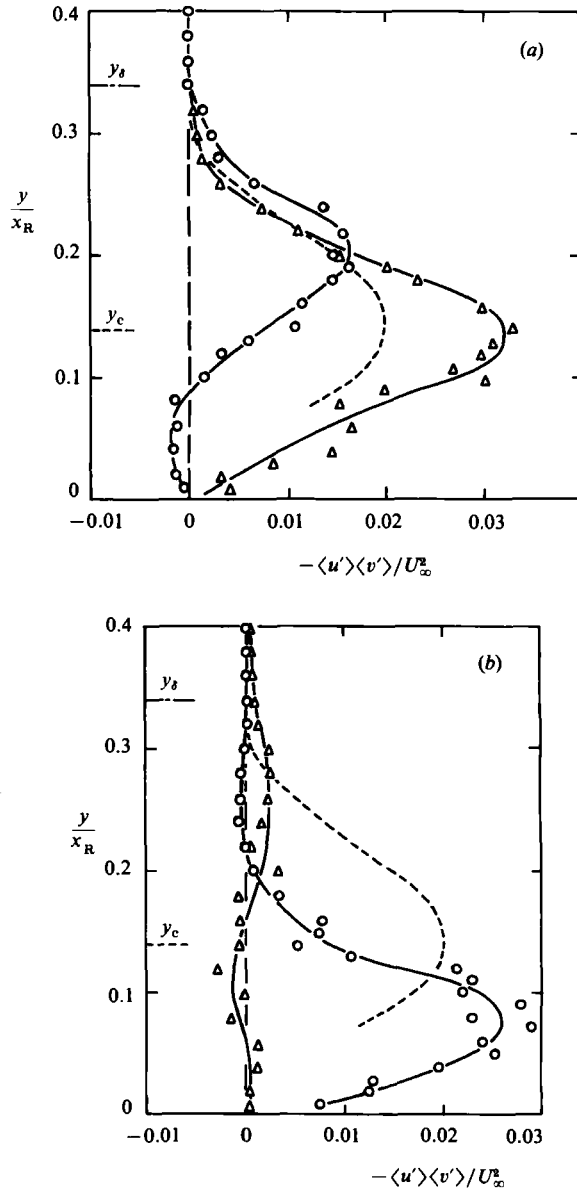
FIGURE 9. Distribution of product \langle u' \rangle \langle v' \rangle in the reattachment section x/x_R = 1.0 : —, global Reynolds shear stress -u'v'/U_\infty^2 ; (a) velocity correlation at the time of peaks (O) and valleys ( \Delta ) of p'_R ; (b) velocity product at the time of peaks (O) and valleys ( \Delta ) of dp'_R/dt . Threshold levels for p'_R and dp'_R/dt were the same, see captions of figures 4 and 5. The frequency of detection of the peaks and valleys of dp'_R/dt was 82 Hz and 110 Hz, respectively.
